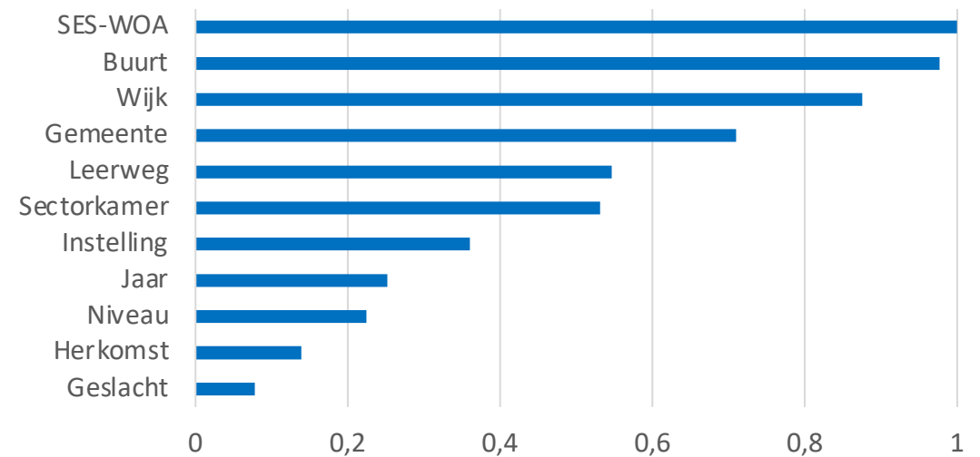
Feature Importance
