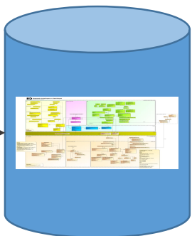
RIO register
